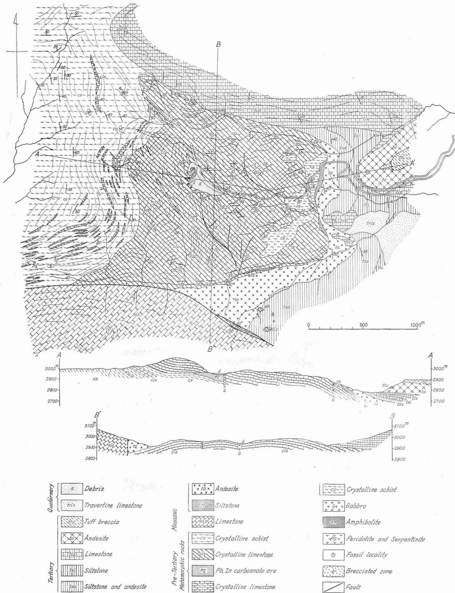
Fig. 2 General geological map and sections of Anguran area.
