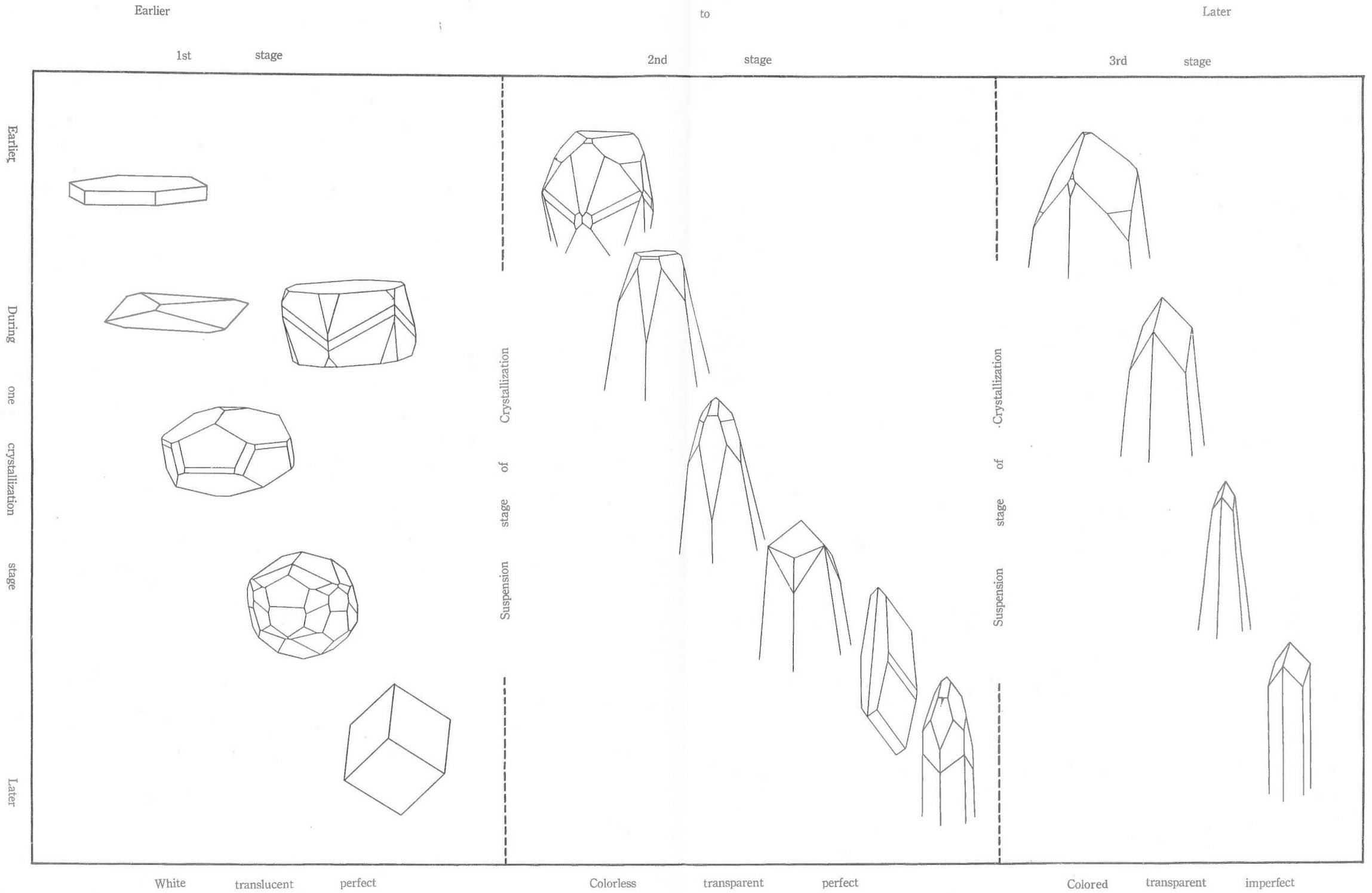
Fig. 4. Sequence of variation in crystal habit of Calcite from Fukuhara according to crystallization stage
