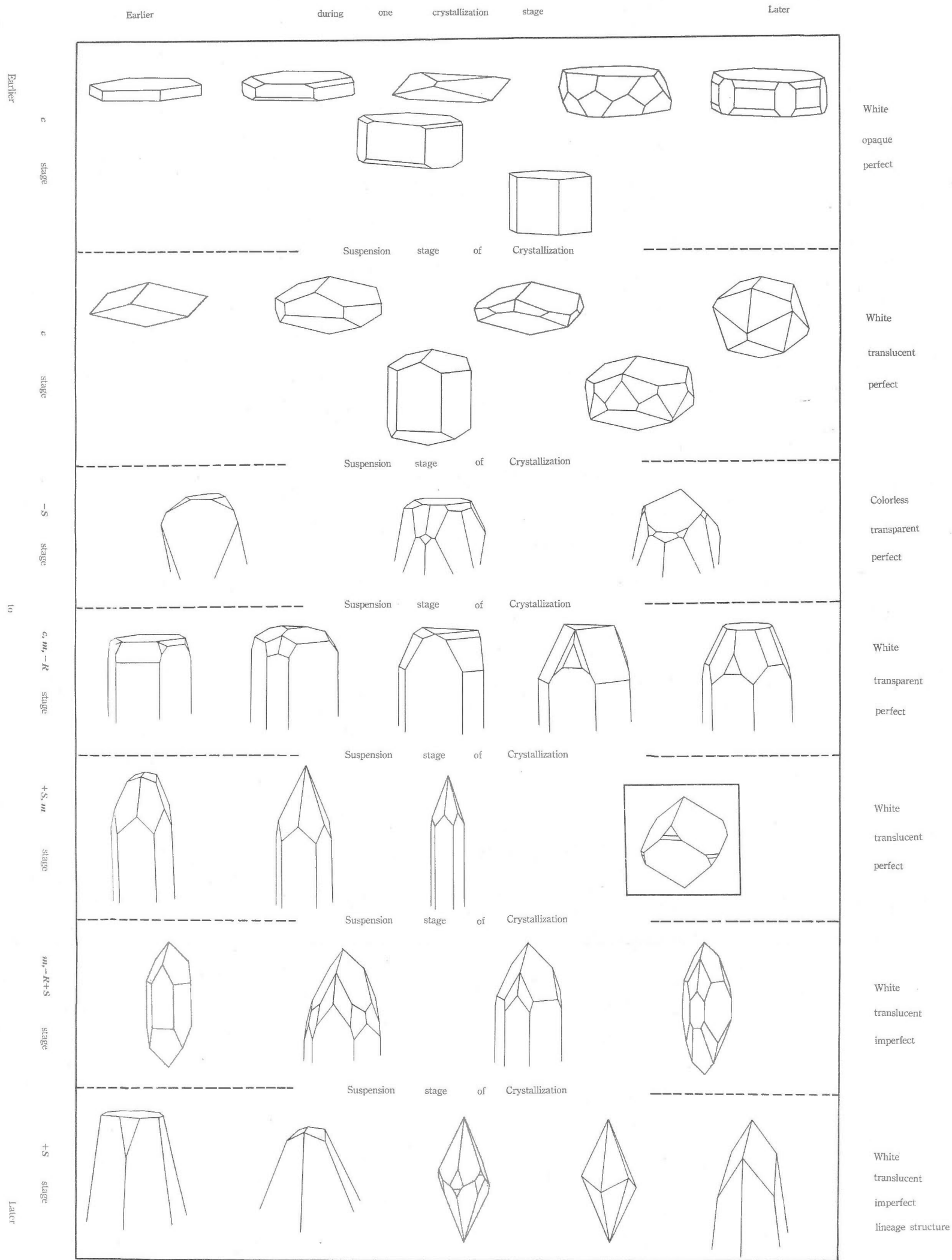
Fig. 8. Sequence of variation in crystal habit of Calcite according to crystallization stage (Ashio mine)
