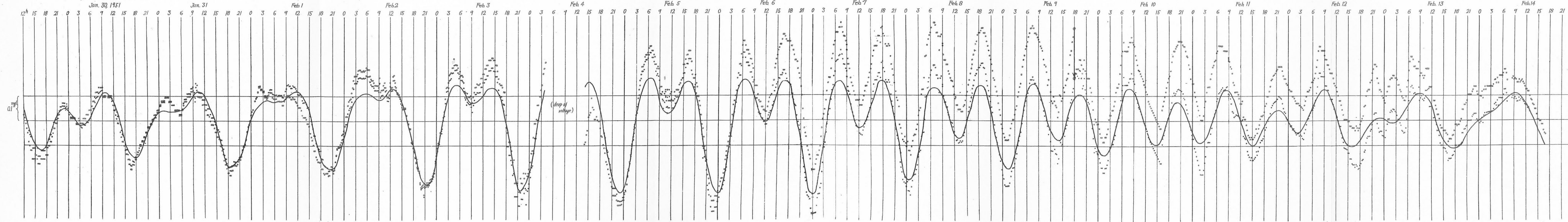
Gravity measurement from Jan. 29 to Feb. 14, 1951 at the Geological Survey of Japan Kawasaki, Japan.
