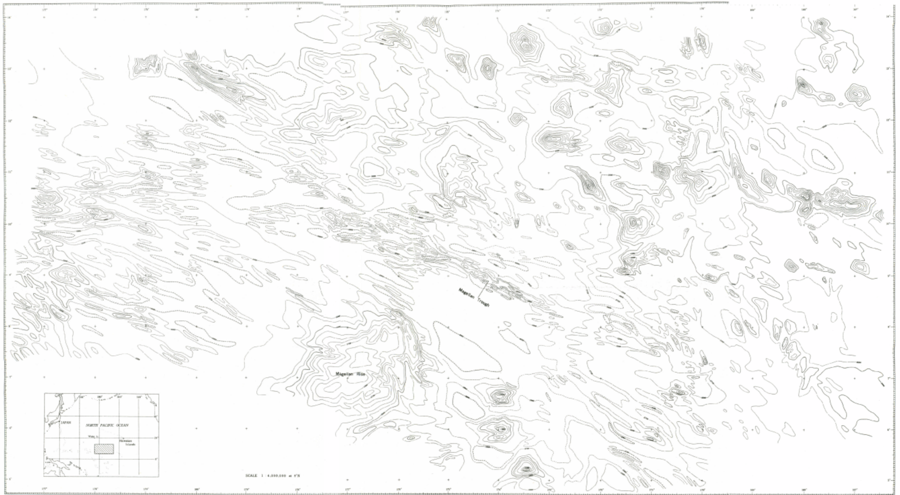
Bathymetric Chart of the Northern Central Pacific Basin.
