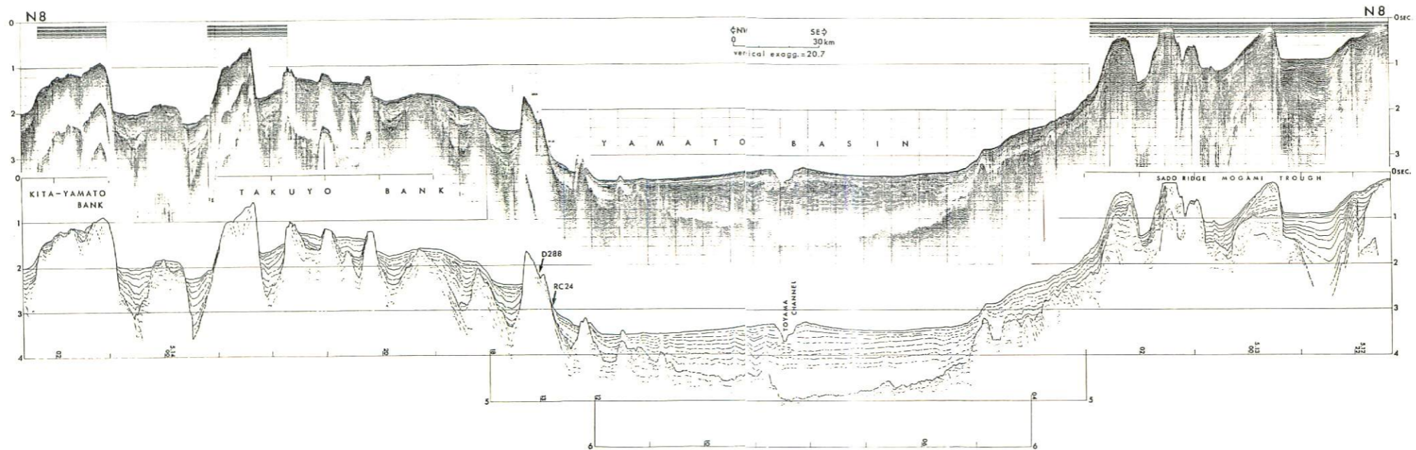
Fig. VI-4 Seismic profiler record of N8 with interpretation.
