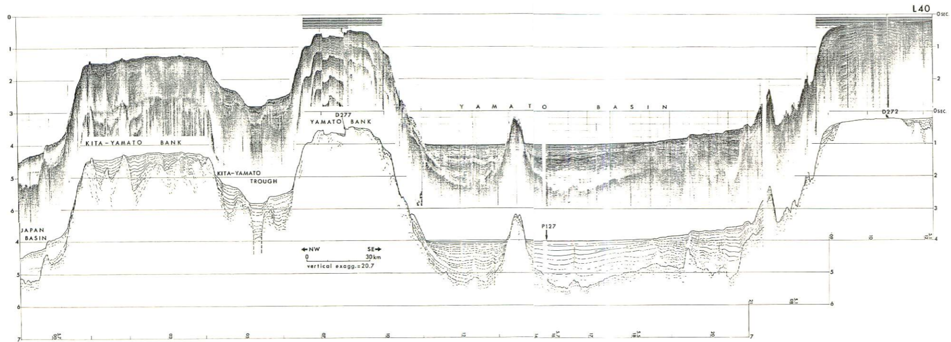
Fig. VI-3 Seismic profiler record of L40 with interpretation.
