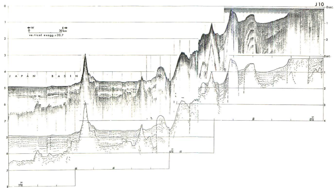
Fig. VI-6 Seismic profiler record of J10 with interpretation.
