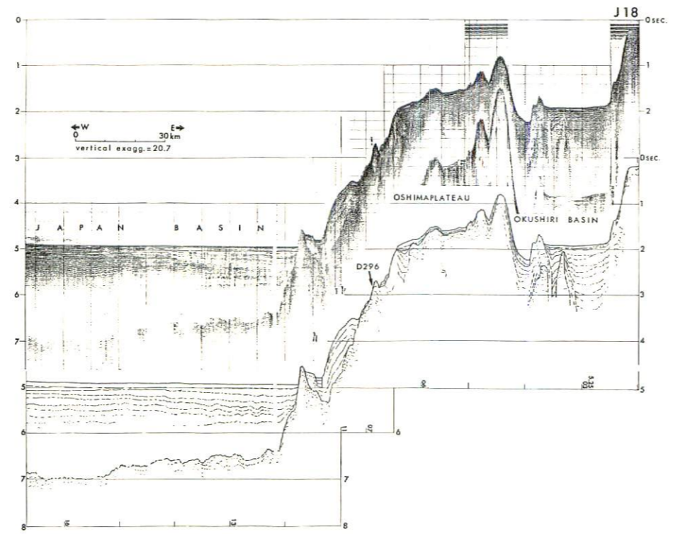
Fig. VI-5 Seismic profiler record of J18 with interpretation.
