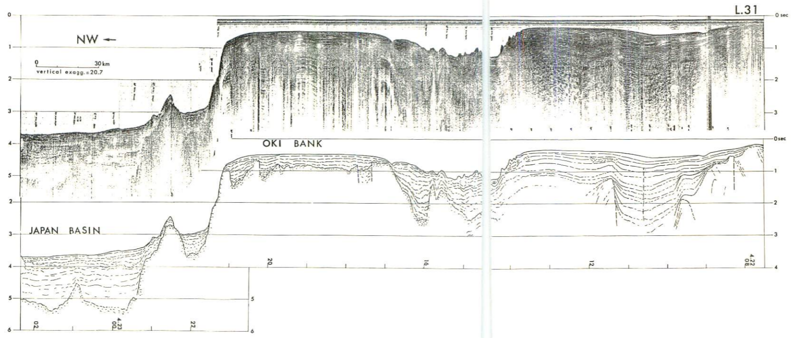
Fig. VI-1 Seismic profiler record of L31 with interpretation. Vertical scale is presented in seconds of two-way travel time. The bottom of the profile is annotated with the time in days and hours.
