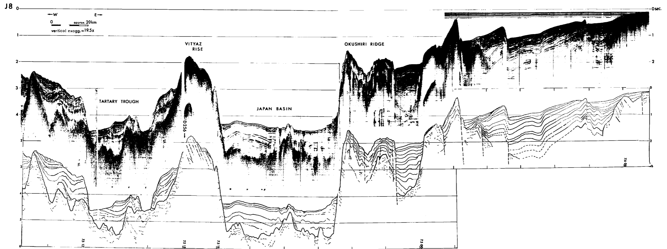
Fig. V-5 Seismic profiler record of J8 with interpretation. Filter: 30~90 Hz.
