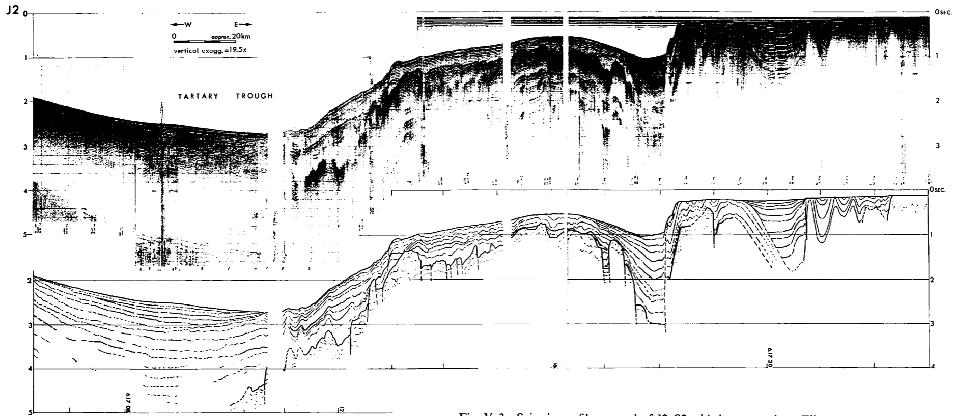
Fig. V-3 Seismic profiler record of J2-S2 with interpretation. Filter: 30~90 Hz.
