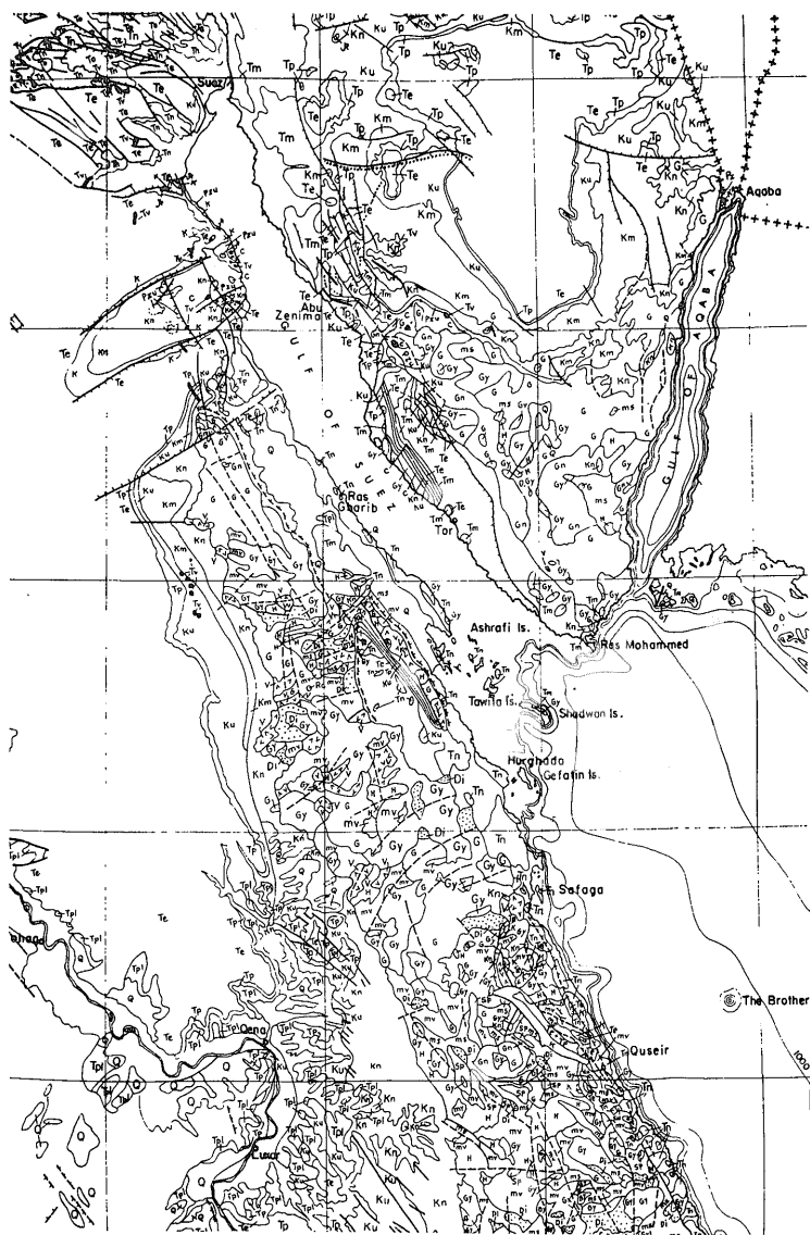
「Geological Map of Egypt」 (The Geological Survey of Egypt, Paper No. 56)
