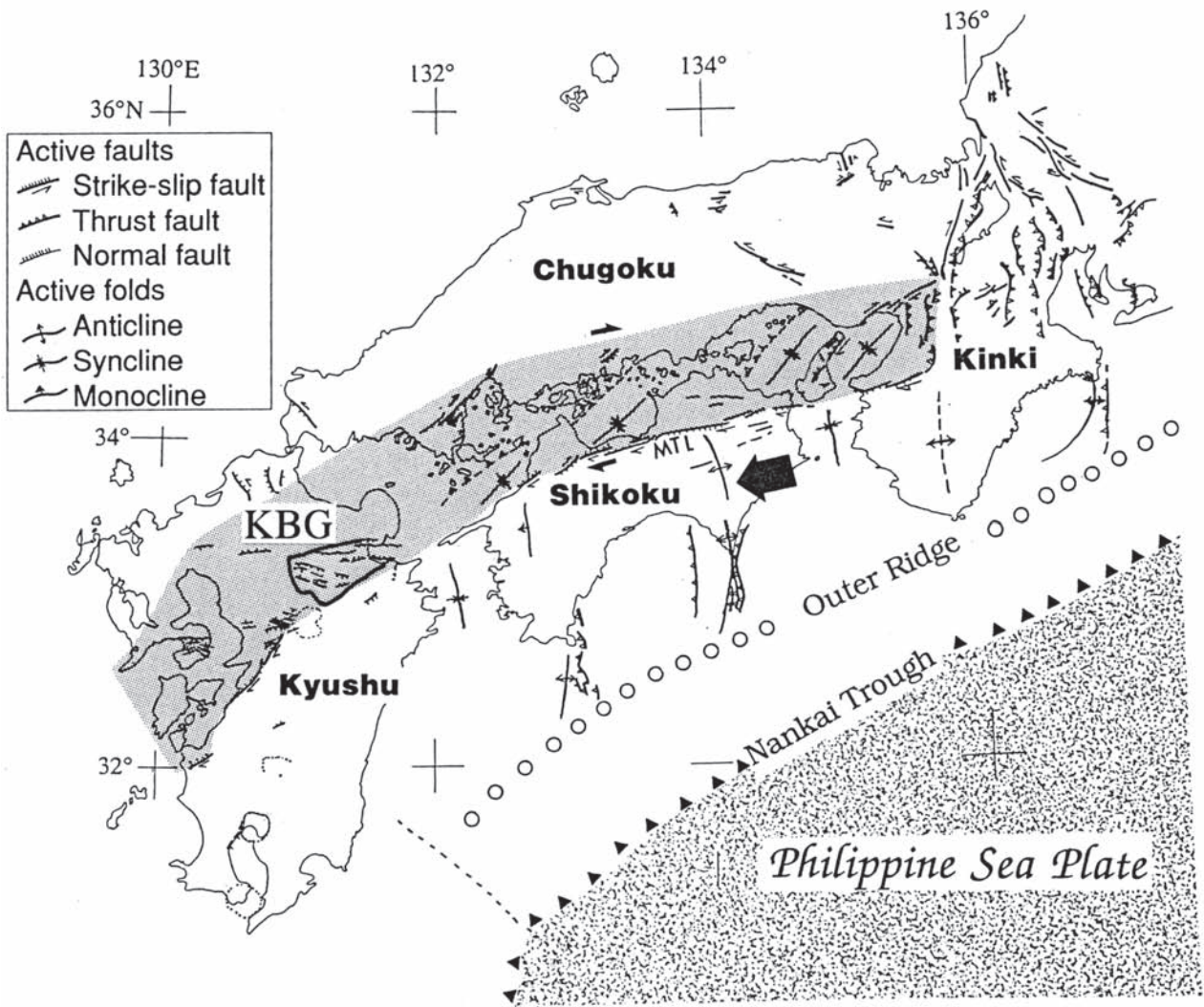
Fig. 1 Tectonic setting of the KBG in terms of oblique subduction of Philippine Sea Plate, after Tsukuda (1993). Solid arrow indicates the direction of the fore-arc translation. Shaded area indicates the right-lateral shear zone (Seto'uchi shear zone). MTL: Median Tectonic Line. The location of the KBG is added by the authors.
