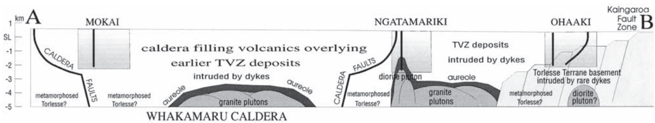
Fig. 7 Schematic cross-section of geologic and thermal structures in the young-TVZ (Wood, 1996). Mokai, Ngatamariki and Ohaaki geothermal systems are shown as shaded rectangular boxes in which the deepest drillholes marked as heavy lines. Both ends of cross-section, A and B are shown in Fig. 5.
