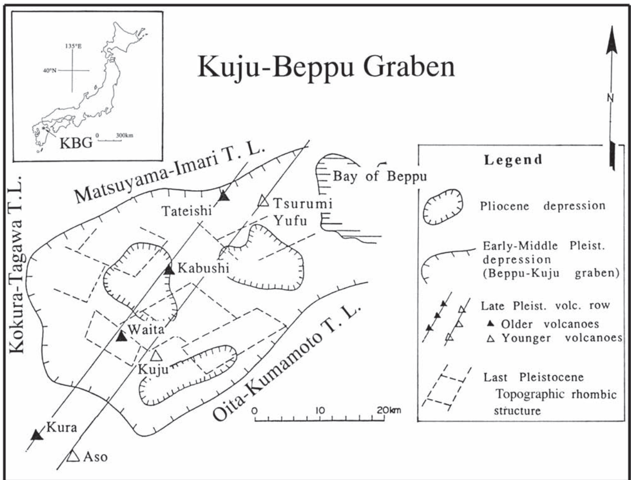
Fig. 3 Principal geologic structures in the KBG (Tamanyu, 1985)
